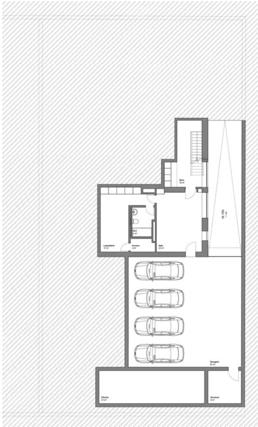
PLANTA PISO -1_civil
